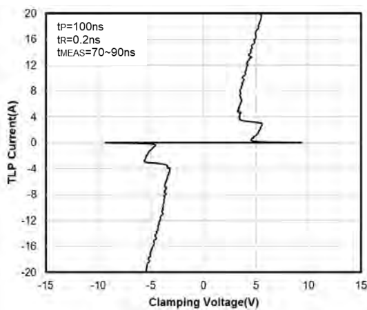
TLP Curve
