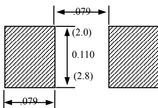
DO-214AA (SMB)
