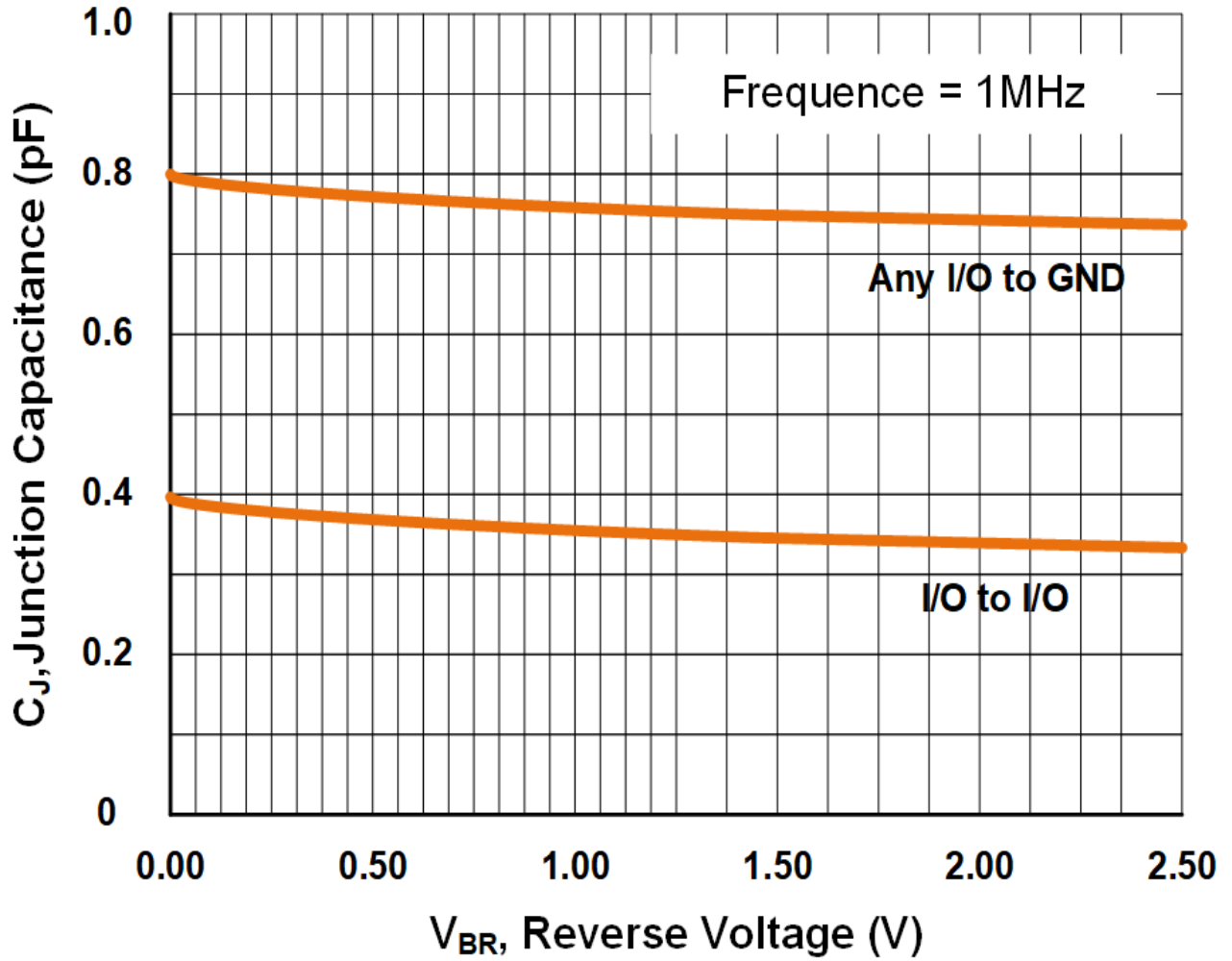
Figure 6. Typical Capacitance vs. Reverse Voltage
