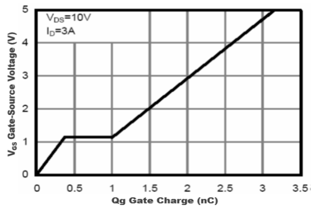
Figure4. Gate Charge
